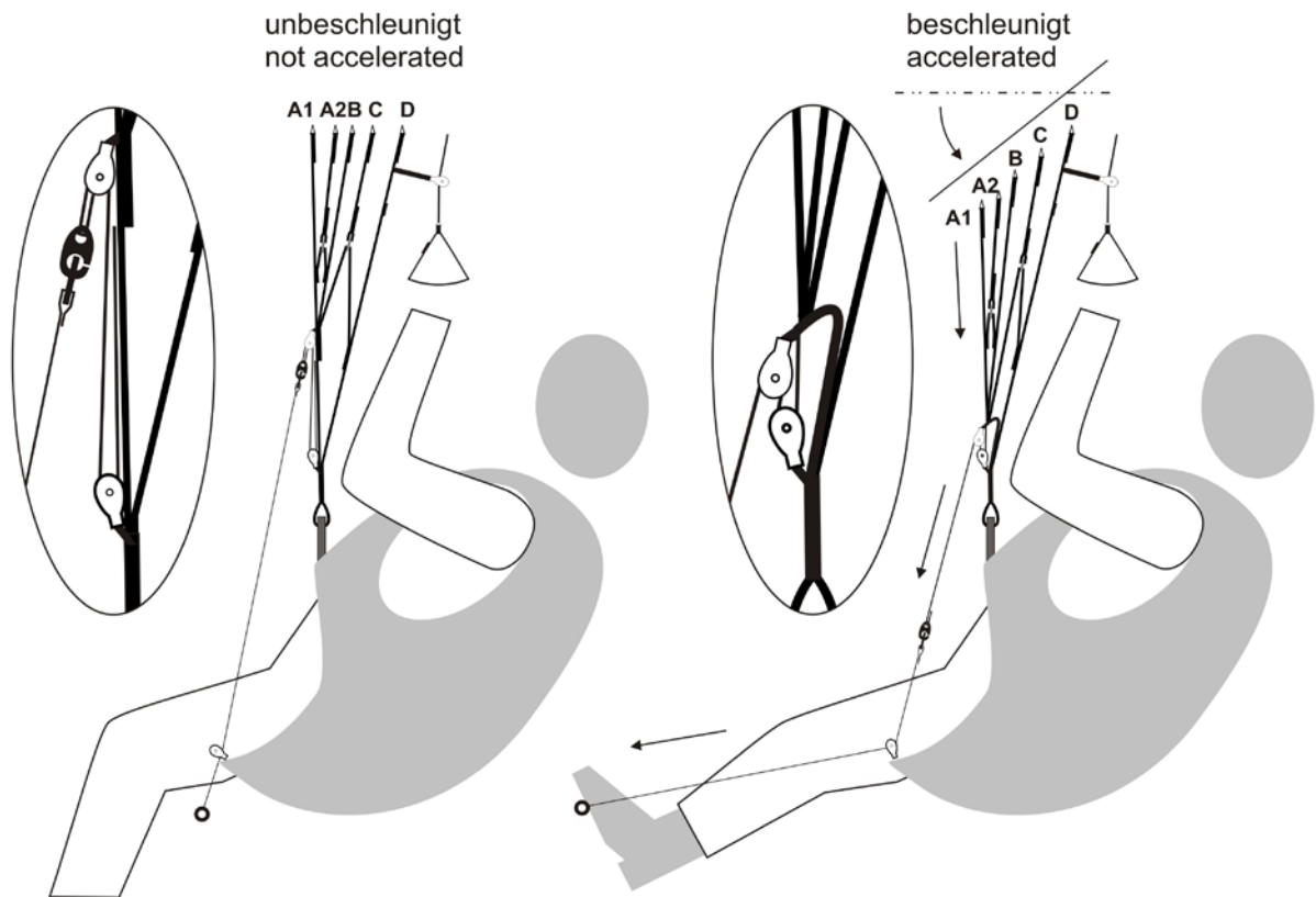
Figure 2: How the Speed system of the ASTRAL 6 works
